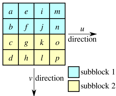
Figure 17.4: Two 4 \times 2 -pixel ETC2 subblocks on top of each other
