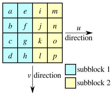
Figure 16.3: Two 2×4-pixel ETC1 subblocks side-by-side
