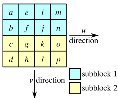
Figure 16.4: Two 4×2-pixel ETC1 subblocks on top of each other
