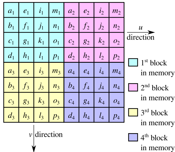
Figure 17.1: Pixel layout for an 8 \times 8 texture using four ETC2 compressed blocks
